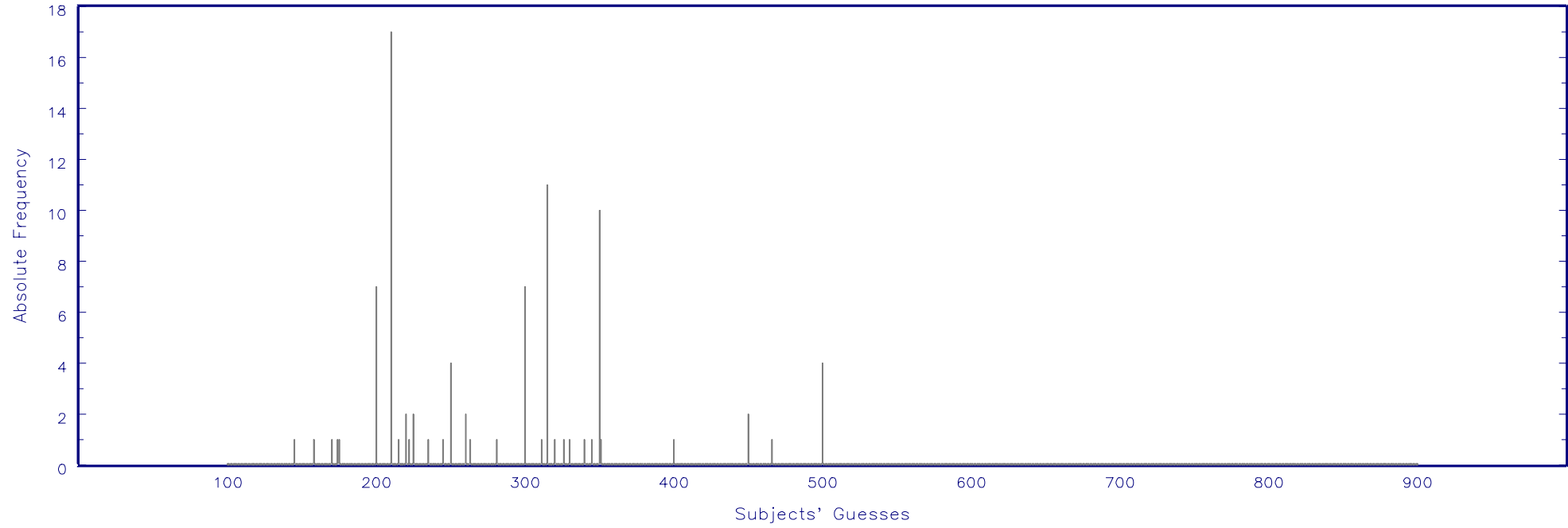
Figure 20: Game 15 - \alpha 2 \alpha 4 - [100,500],0.7;[100,500],1.5
