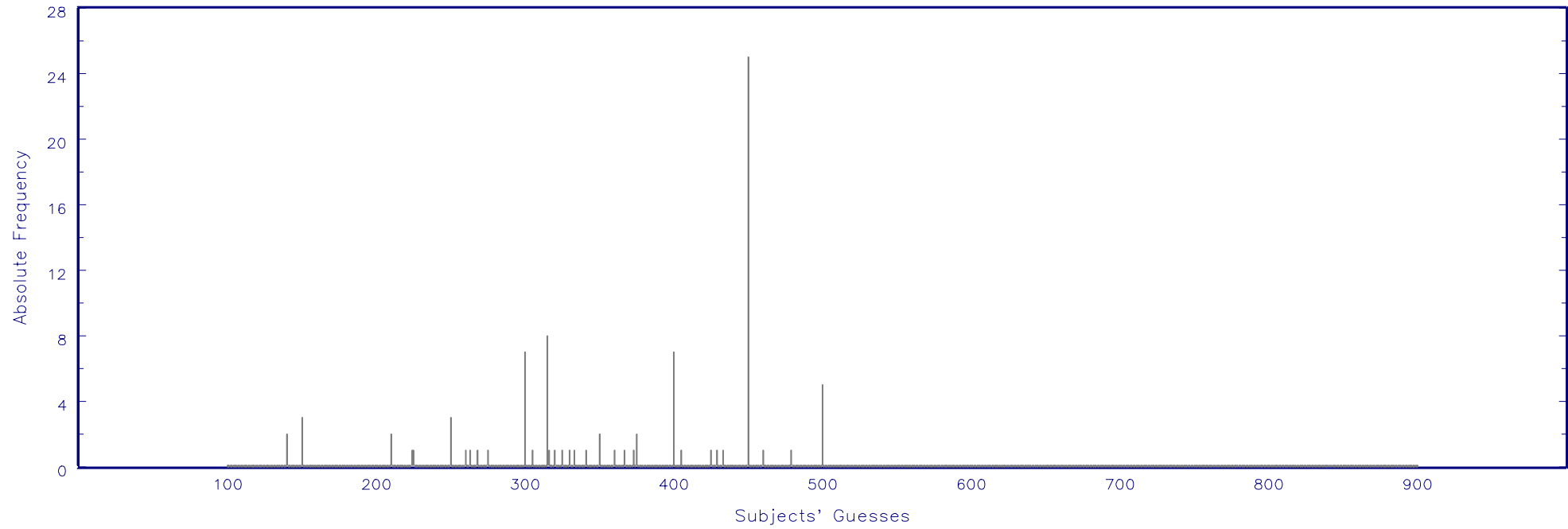
Figure 2P: Game 16 - \alpha 4 \alpha 2 - [100,500],1.5;[100,500],0.7
