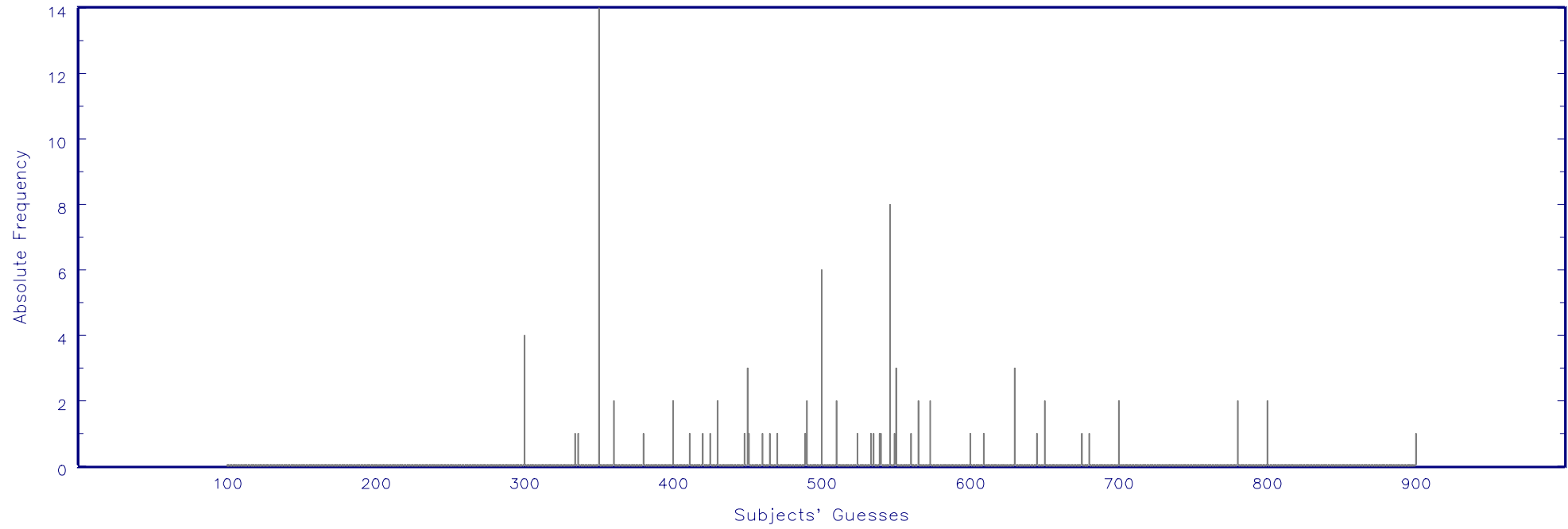
Figure 2K: Game 11 — \delta\beta 3 — [300,900],0.7;[100,900],1.3
