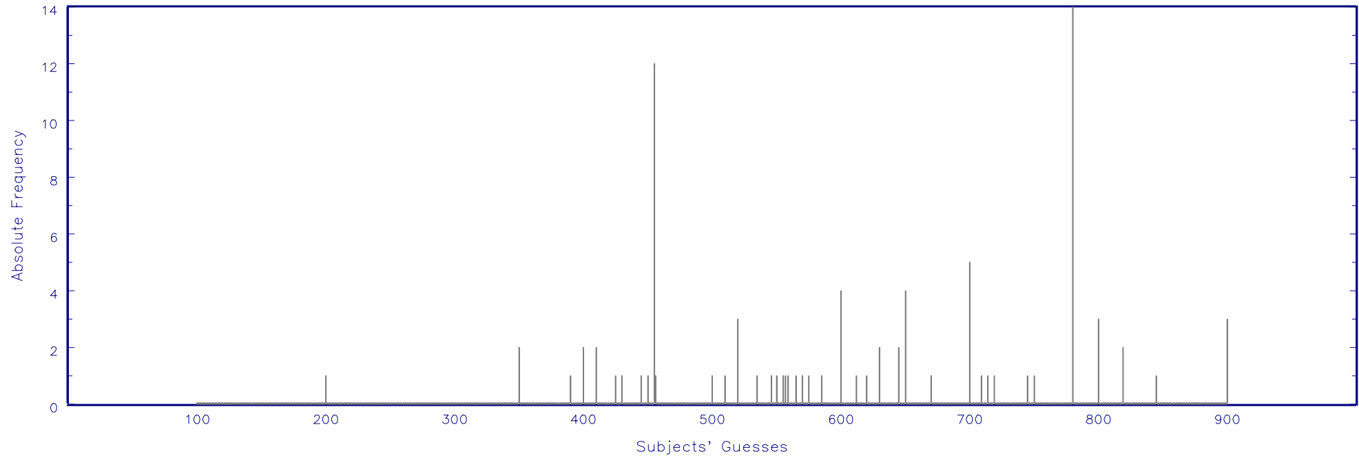
Figure 2L: Game 12 — \beta 3\delta 2 — [100,900],1.3;[300,900],0.7
