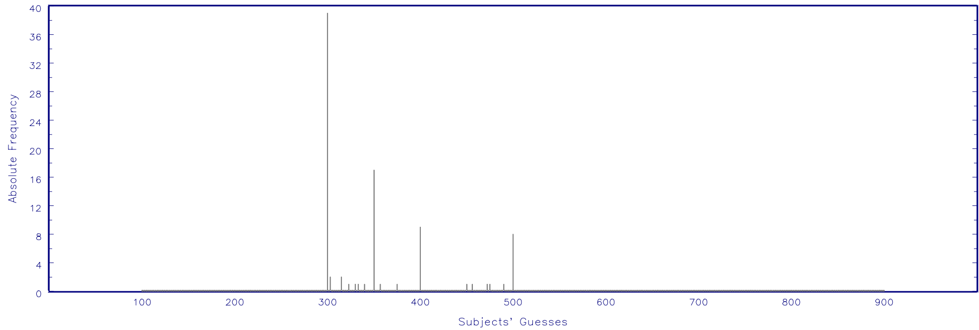
Figure 2D: Game 4 - \gamma_2\beta_1 - [300,500],0.7;[100,900],0.5
