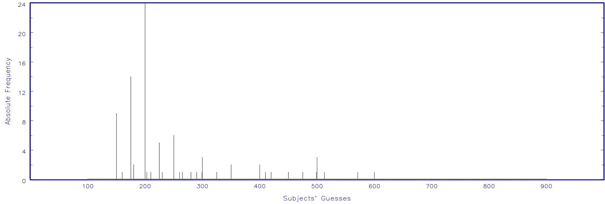
Figure 2C: Game 3 - \beta_1\gamma_2 - [100,900],0.5;[300,500],0.7
