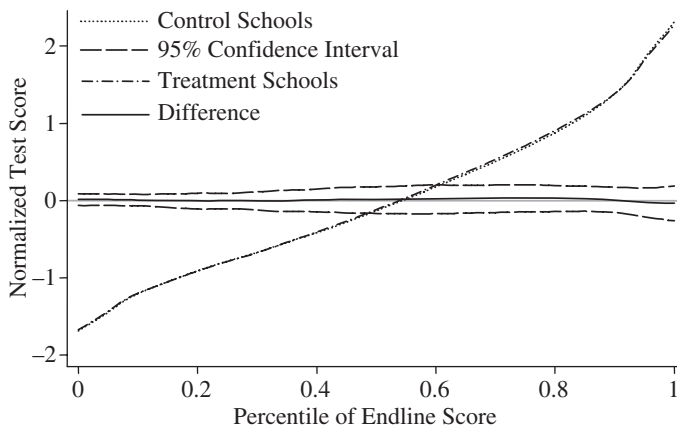
Fig. 2. Quantile (Percentile) Treatment Effects
