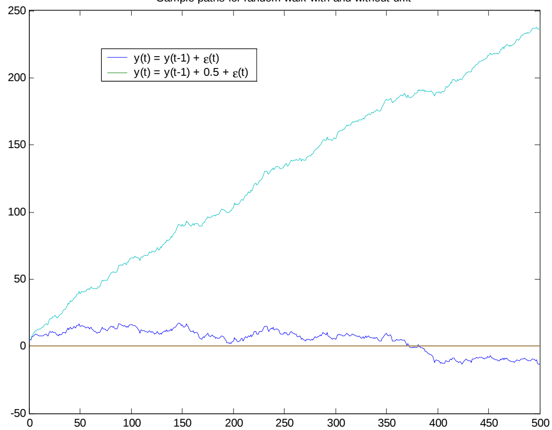
Sample paths for random walk with and without drift
